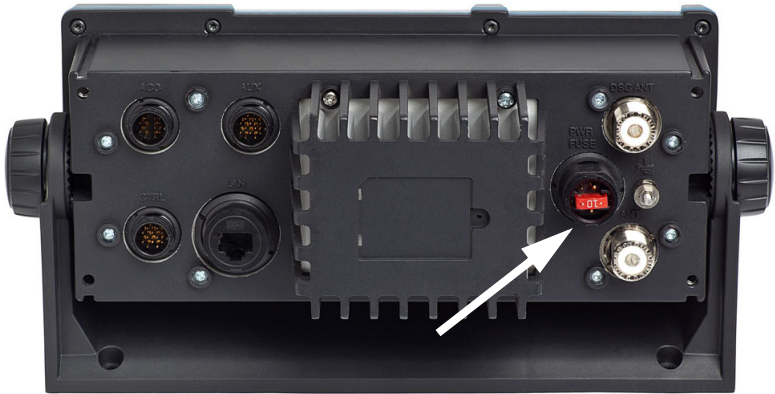
Figure 4: Replacing the fuse in the power connector
